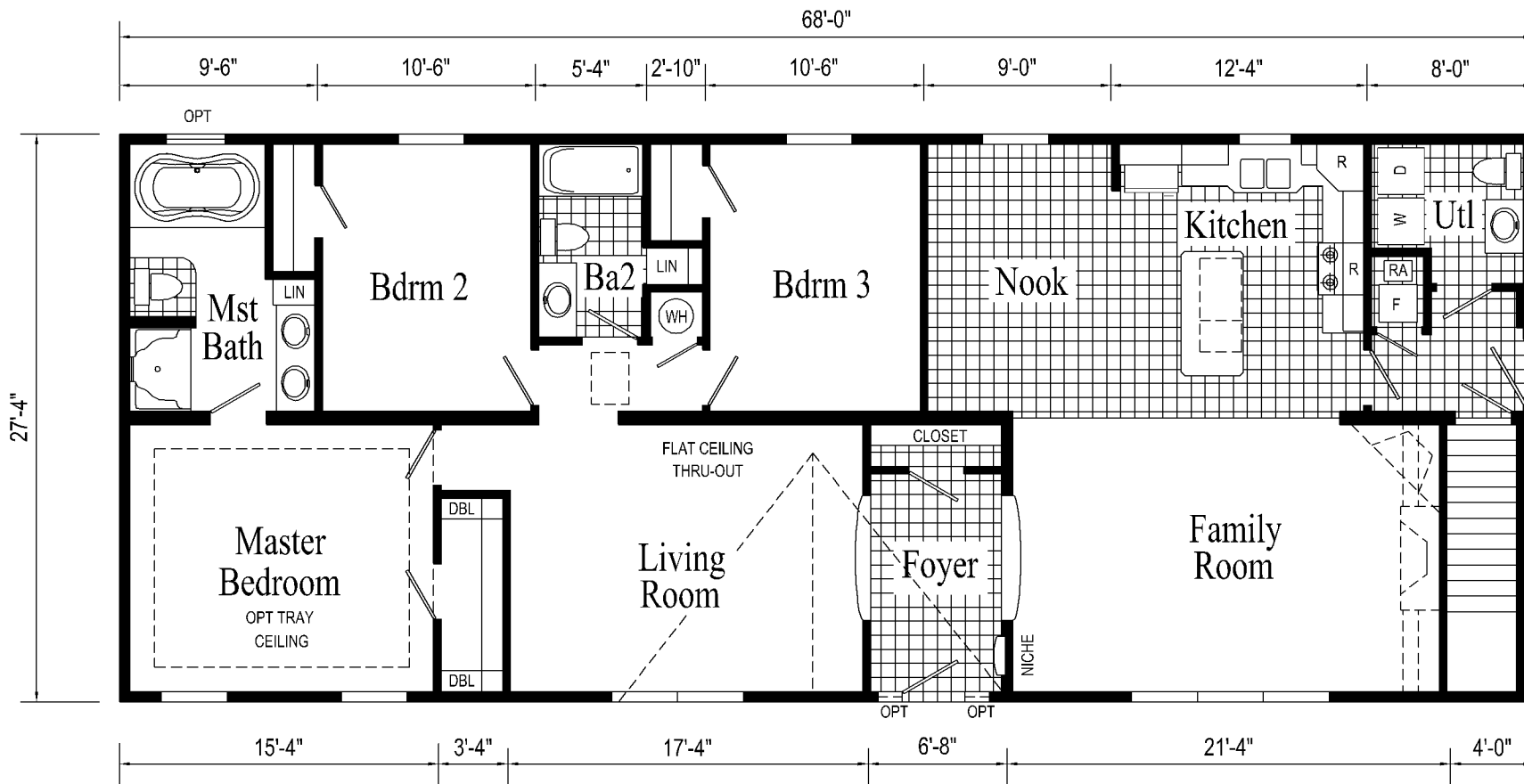
HR104-A 28 x 68 Approx. 1859 Sq. Ft.
