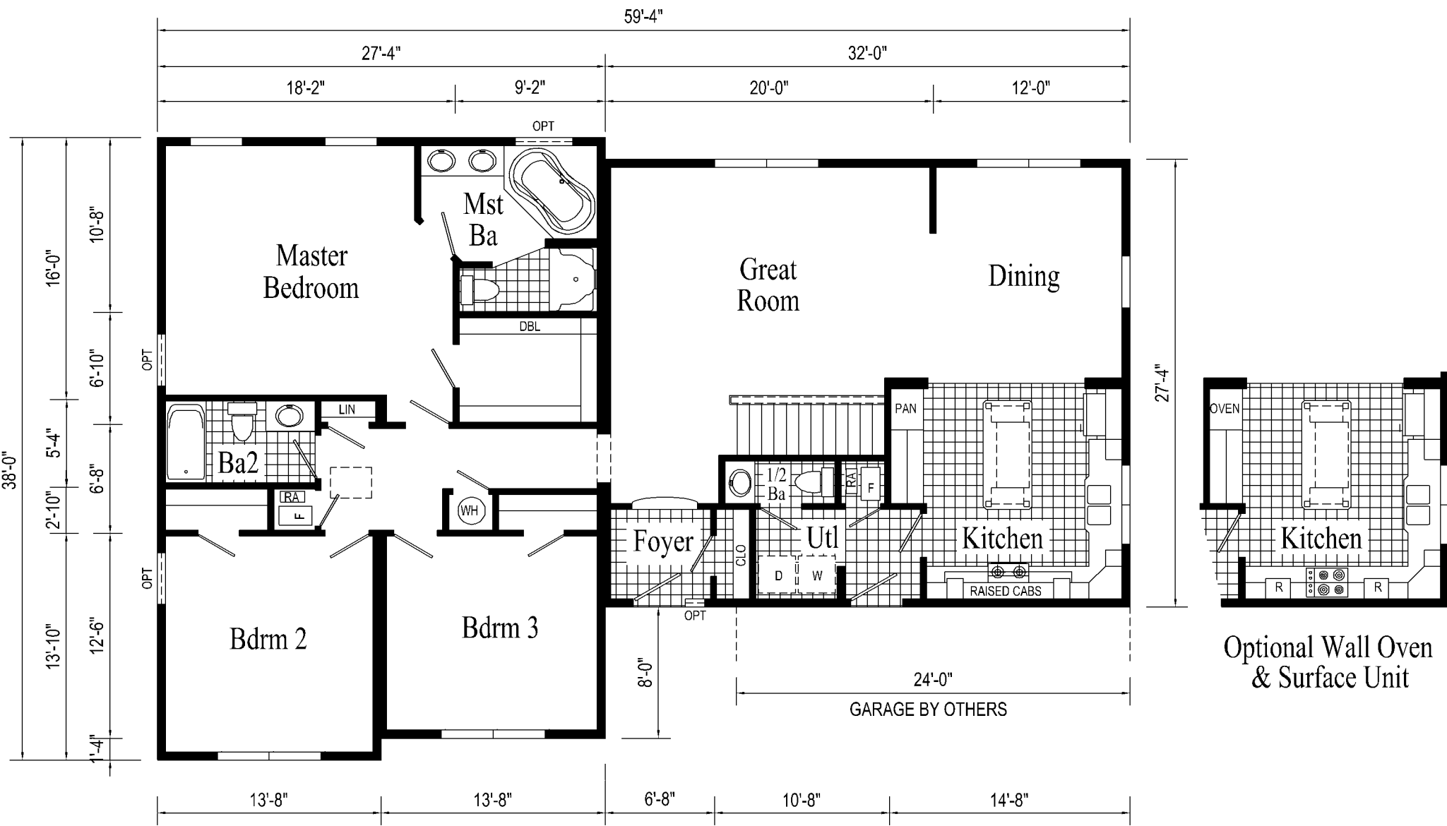
HT103-A 38 X 59-4 Approx. 1895 Sq. Ft.
