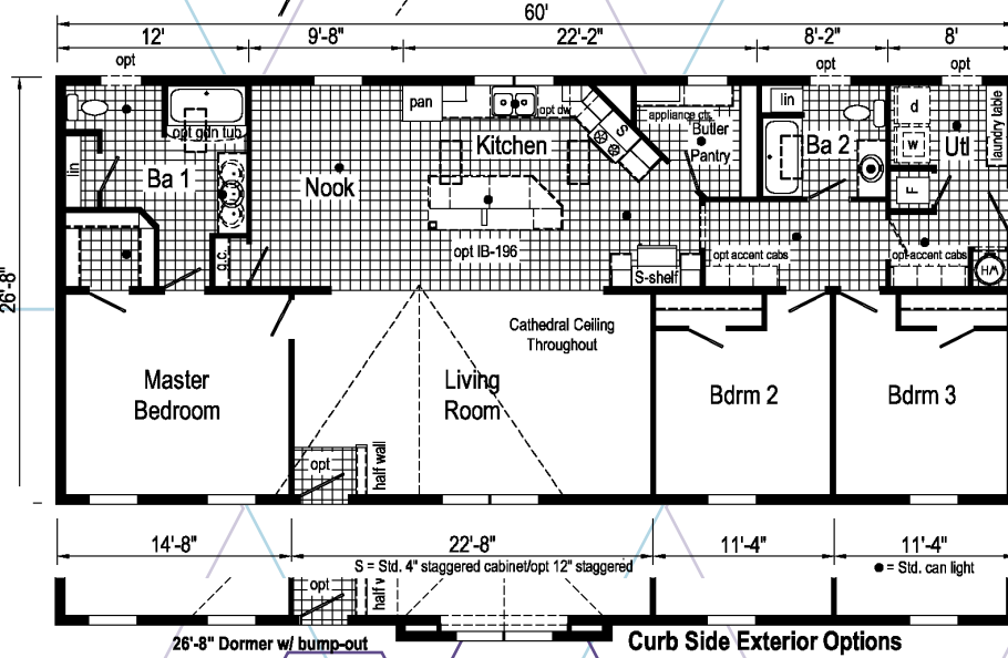
26'-8" Dormer w/ bump-out
